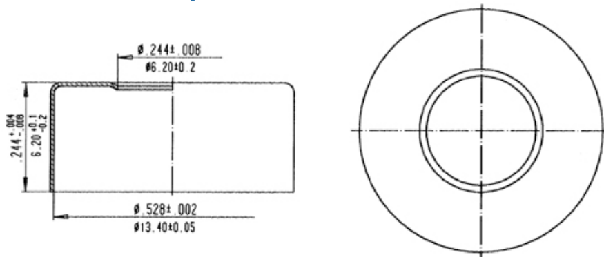
Product: Aluminum Cap 13-0016
